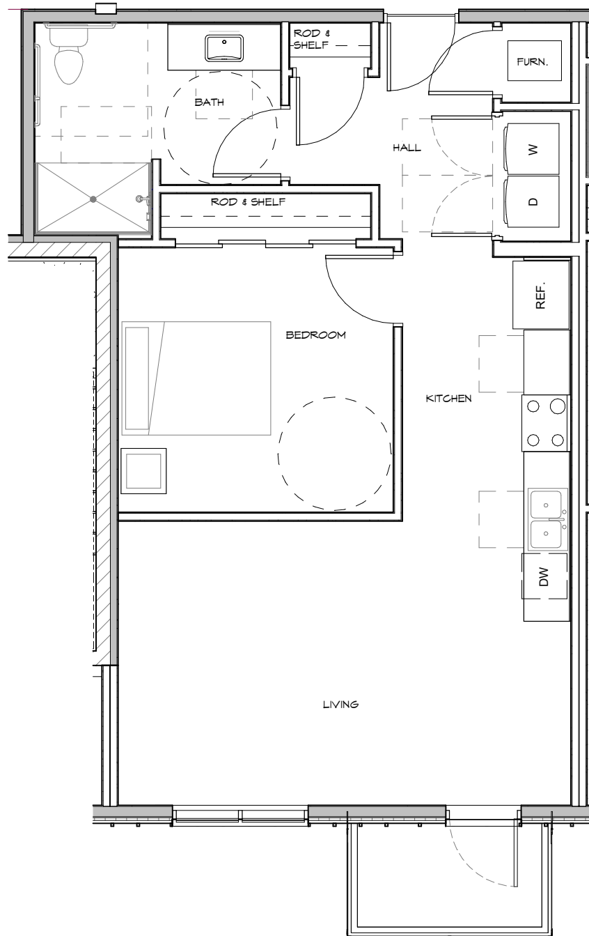
UNIT 407 FLOOR PLAN 726 S.F. & 45 S.F. DECK
