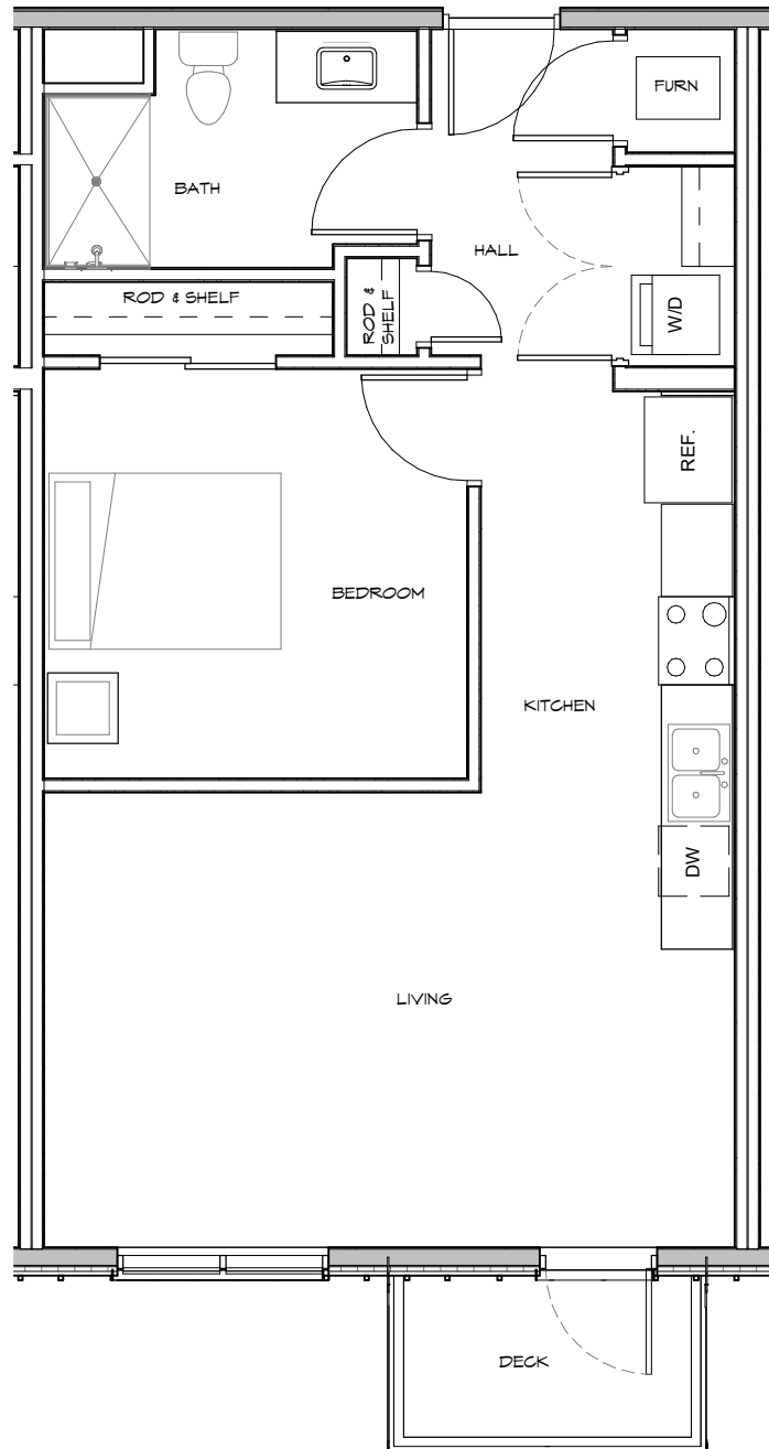
UNIT 404, 405, 406, 504, 505 & 506 FLOOR PLAN 678 S.F. & 45 S.F. DECK
