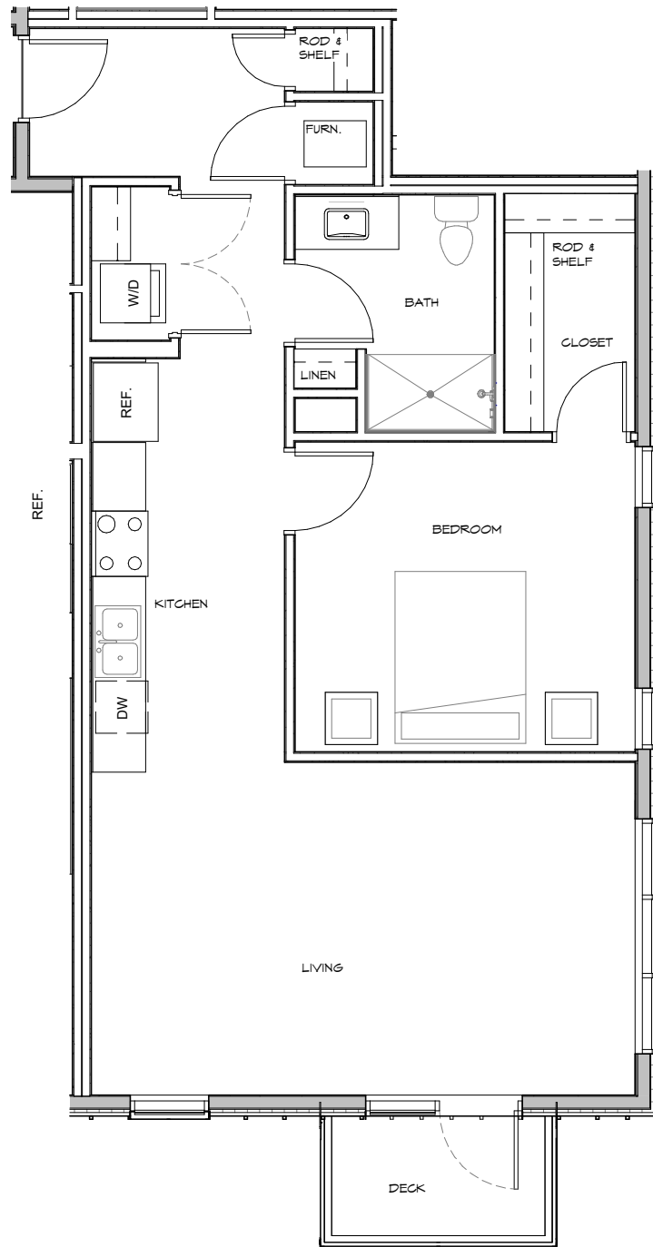
UNIT 403 & 503 FLOOR PLAN 800 S.F. & 45 S.F. DECK
