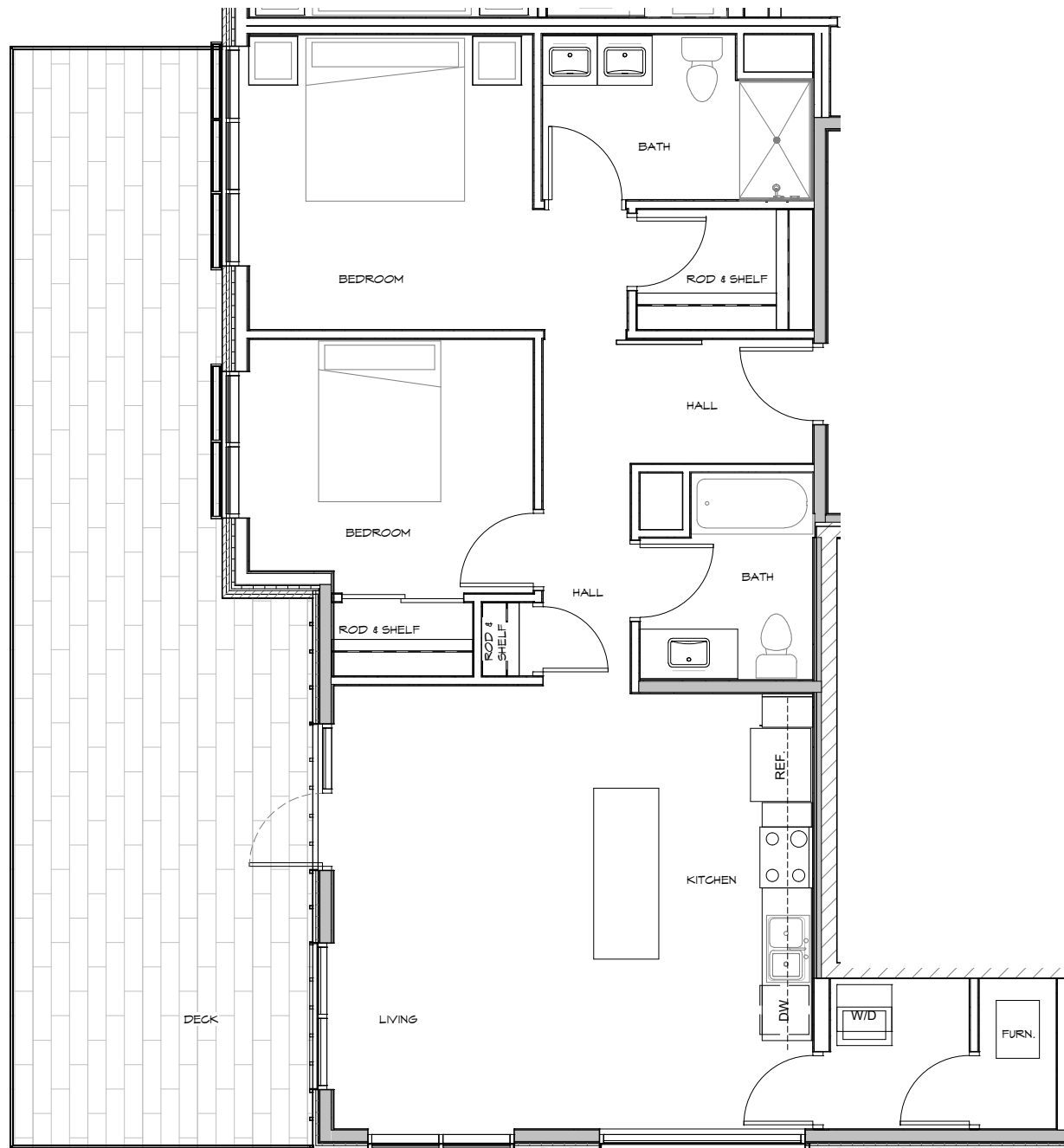
UNIT 308 FLOOR PLAN 1,018 S.F. & 477 S.F. DECK
