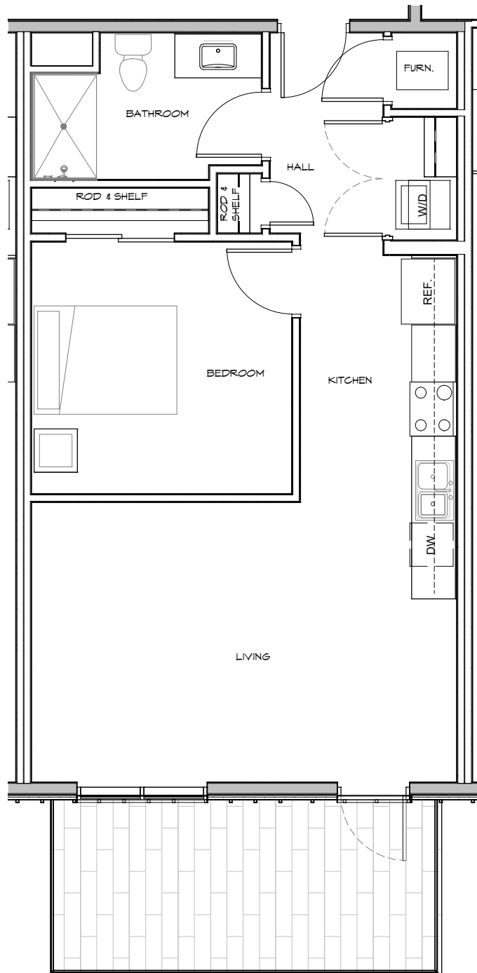
UNIT 304, 305, & 306 FLOOR PLAN 678 S.F. & 144 S.F. DECK
