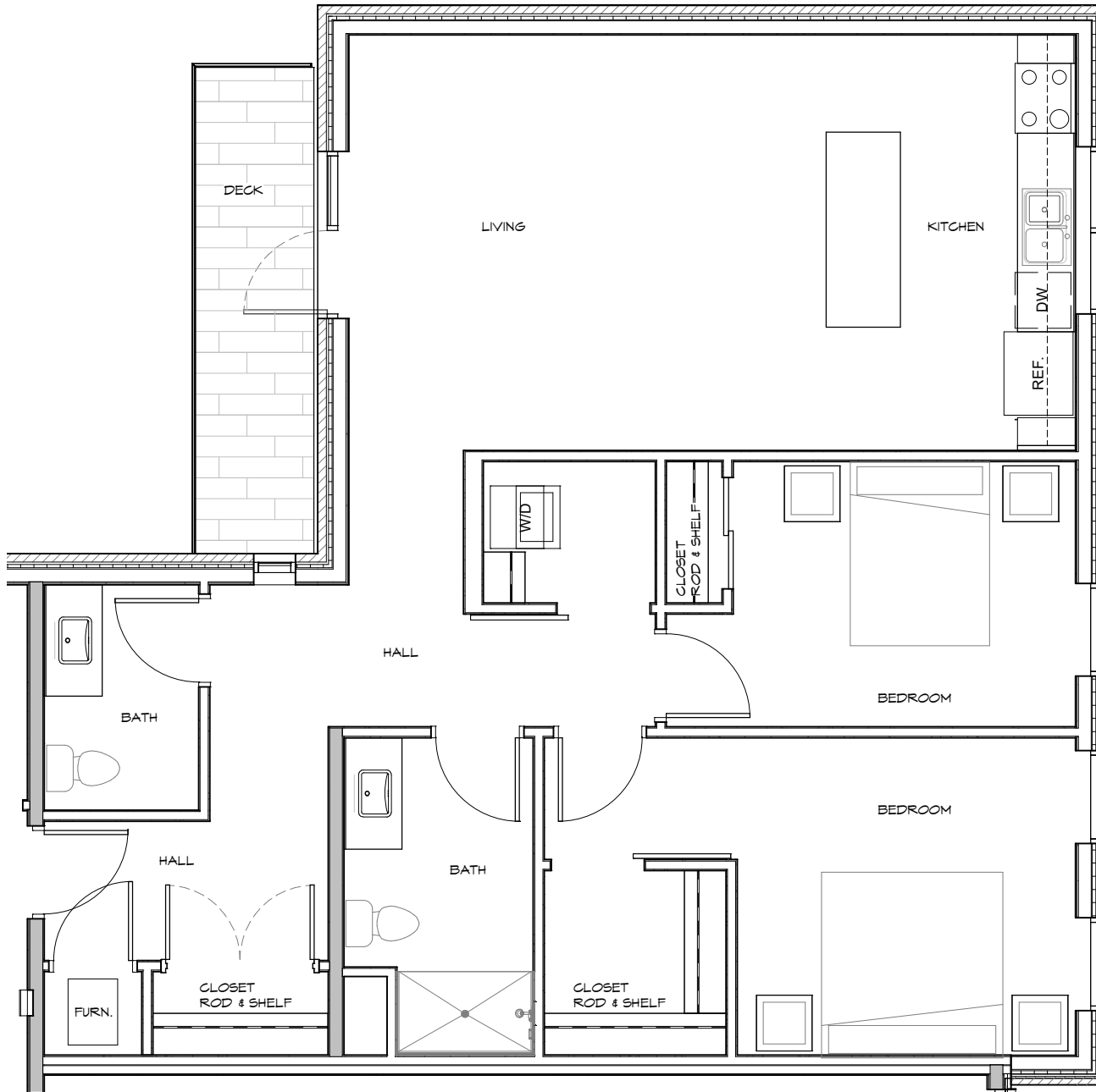
UNIT 301 FLOOR PLAN 1,139 S.F. & 74 S.F. DECK
