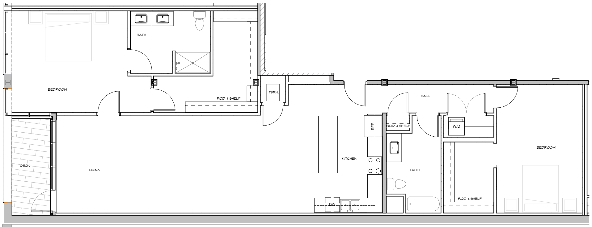
UNIT 206 FLOOR PLAN 1,702 S.F. + 73 S.F. DECK
