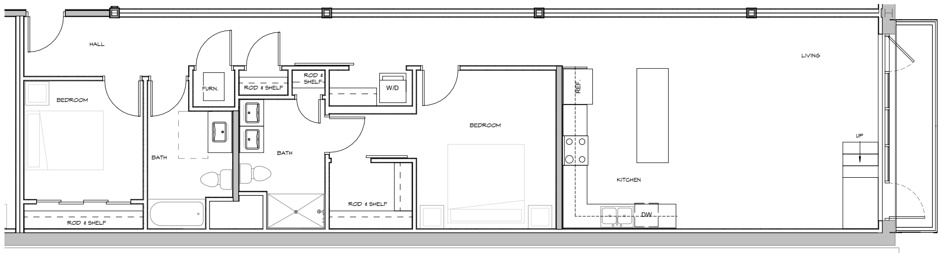
UNIT 205 FLOOR PLAN 1,298 S.F. & 65 S.F. DECK
