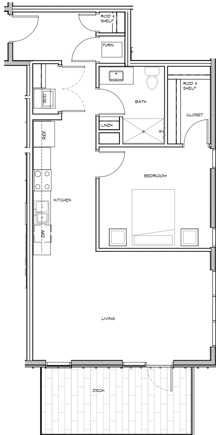
UNIT 303 FLOOR PLAN 800 S.F. & 144 S.F. DECK
